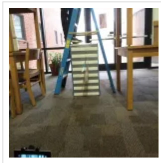
Bungee drop test. Note the iPad recording using a slow motion stop action app.
